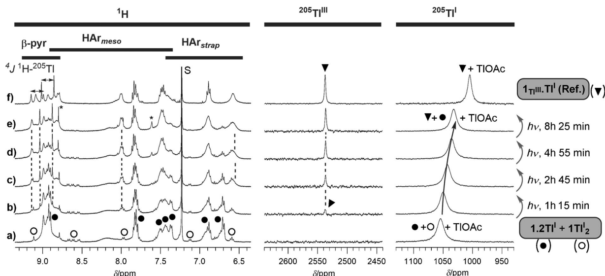
Figure 4. a) ^1\text{H} (left) and ^{205}\text{Tl} (right) NMR spectra of a mixture of 1\cdot 2\text{Ti}^{\text{III}} and 1\text{Ti}^{\text{II}}_2 , formed by the addition of five equivalents of TIOAc to 1 . Conditions: \text{CDCl}_3/\text{CD}_3\text{OD} (9:1), 298 K, DIPEA (10 equiv). b–e) Evolution of the NMR spectrum upon exposure of the NMR tube to indirect sunlight for approximately 8 hours, showing the gradual apparition of 1\text{Ti}^{\text{III}}\cdot\text{Ti}^{\text{I}} (Scheme 2, pathway B). f) Reference spectra of a sample of 1\text{Ti}^{\text{III}}\cdot\text{Ti}^{\text{I}} that was formed by the addition of \text{Ti}(\text{OAc})_3 (1.25 equiv) and TIOAc (5 equiv) to 1 (Scheme 2, pathway A). S = solvent, * = impurity.
